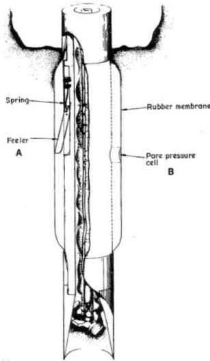
Figure 1: the pressuremeter used (Clarke et al. 1979)
