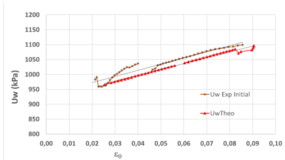
Figure 4: Plastic behaviour - Experiment & Theory: Evolution of effective pressure as a function of orthoradial deformation
