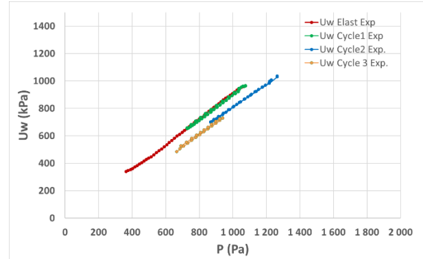
Figure 1: Elastic behaviour - Determination of B_{\text{pres}}=0.925 on virgin loading and 3 cycles
